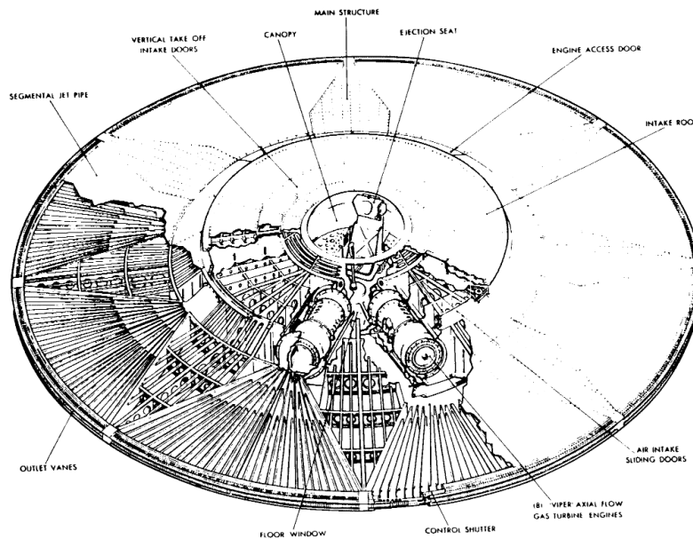
Fig. 2 Cut Away of Research Aircraft
